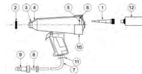
Using the Supplied Nozzle
